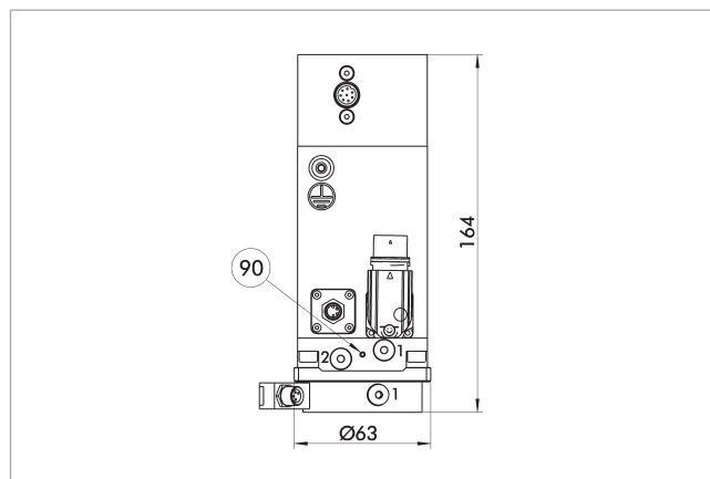
⑨⑩ M3/6 air purge connection
